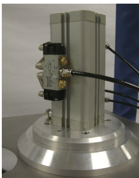
Air Motor of Resin Pump
