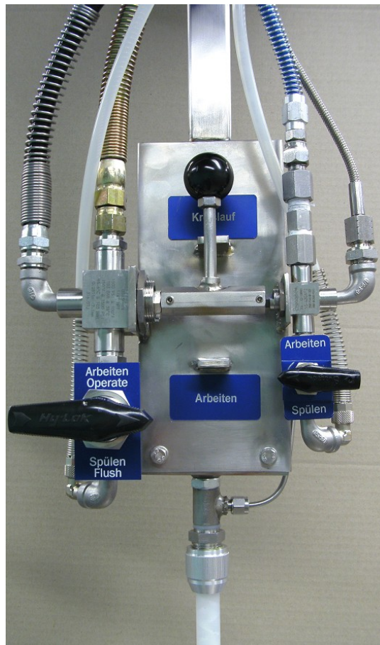
RTM mixing head
